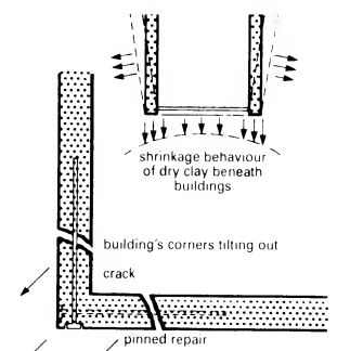
⑬ Pinning of a tilting corner
